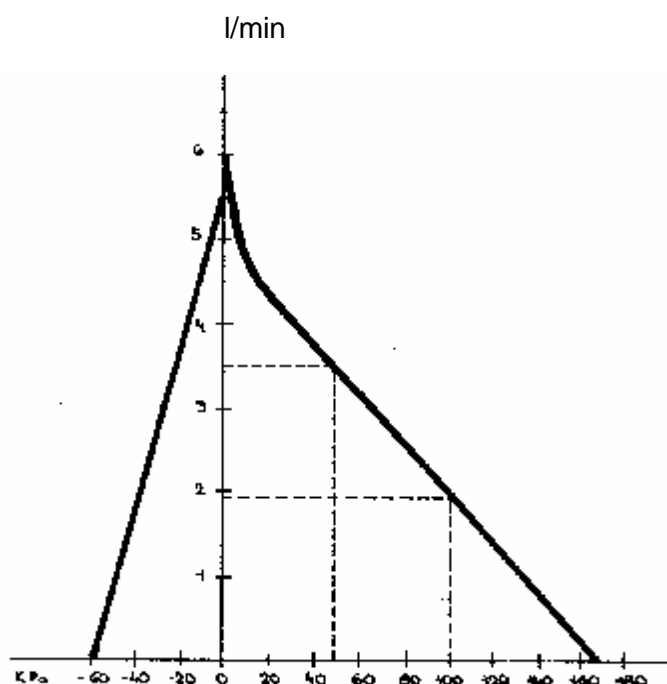
Informative power curve of pump
